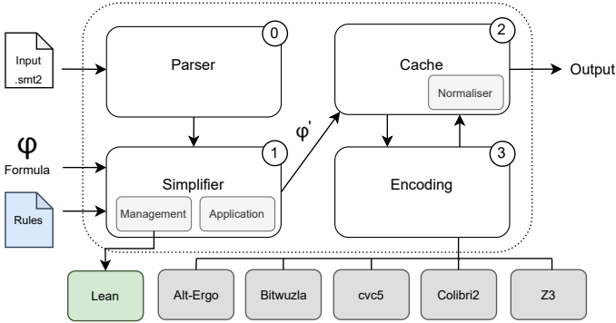
Fig. 1: Overview: Architecture of SMT.ML.
